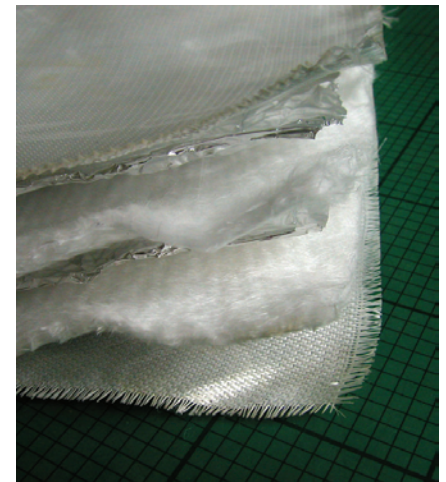
3 foil layers interleaved with high temperature glass fibre construction
