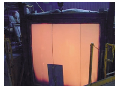
FlameStop60 during fire testing
